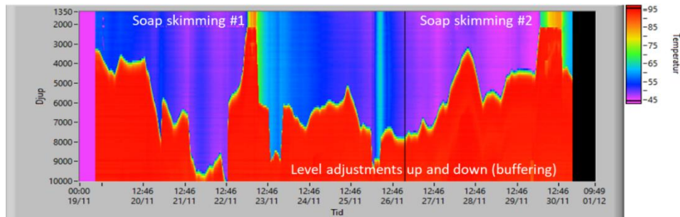
Time series data showing the soap layer movements during the skimming process.
