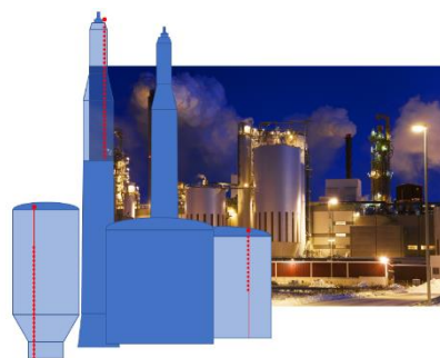
Fiber optic array sensing potential probe locations in the Kraft pulping process: the lower 2/3 of filtrate tanks; the top section of a digester; and in the upper half of decantation tanks for tall oil extraction.
