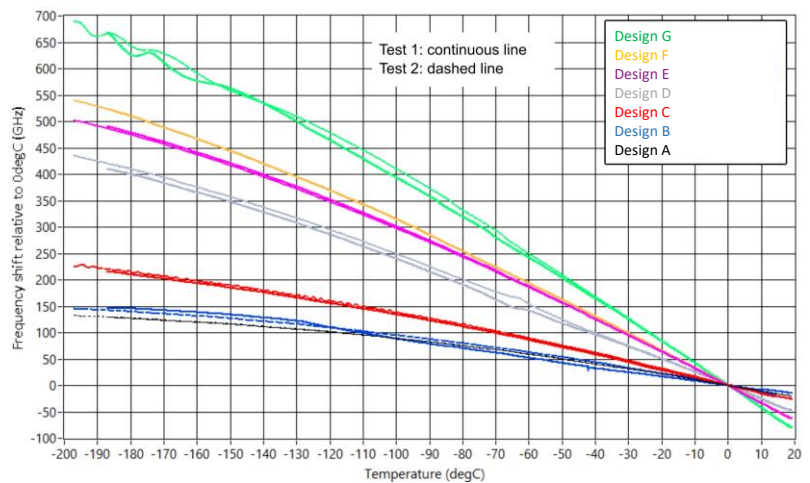
Proximion screening test of the wavelength responses vs. temperature down to minus 196°C (77K) for various bare, coated and encapsulated fiber combinations.
