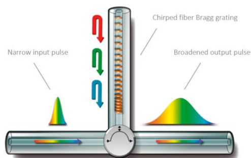
A Proximon CFBG broadens a spectral pulse to emulate chromatic dispersion
